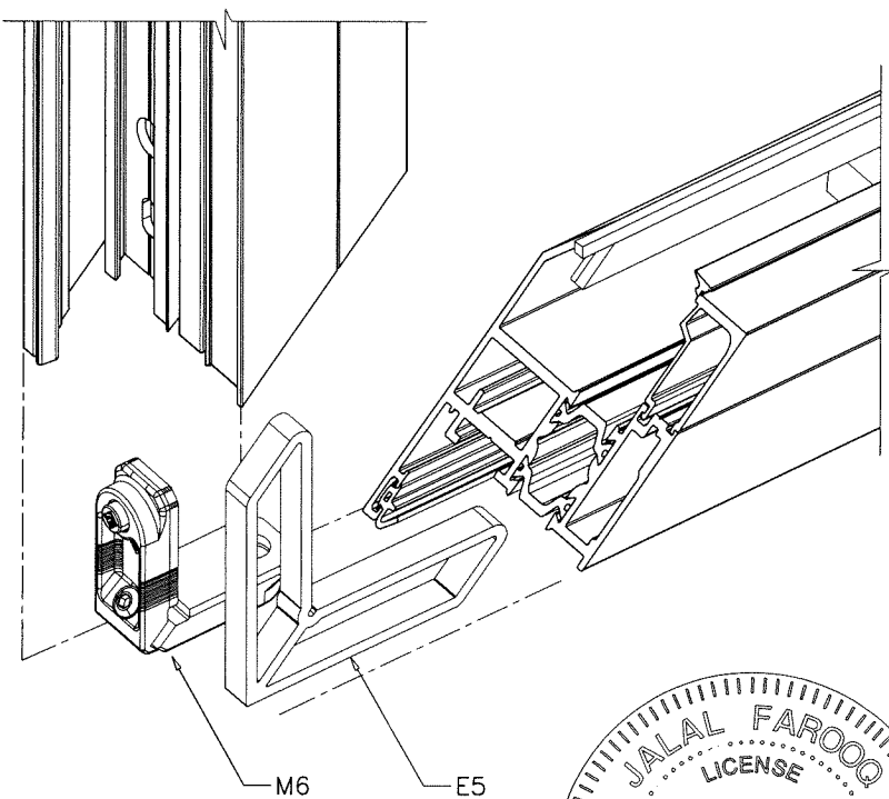
VENT ASSEMBLY
