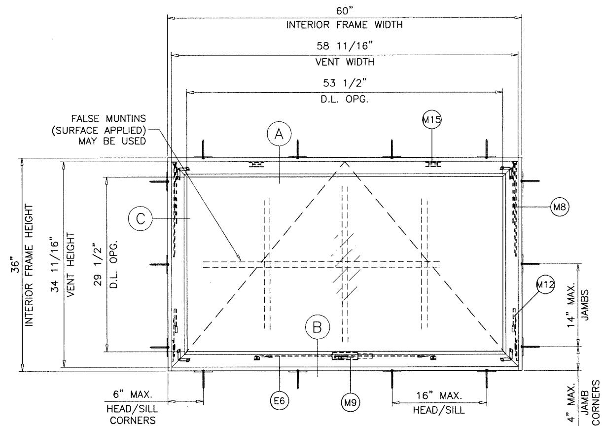
TYPICAL ELEVATION
